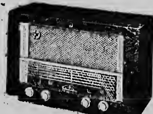
BX 626 U Six wavebands. Six-valve AC/DC receiver. Rotatable Ferroceptor. Flywheel tuning. Infinite short-wave bandspread.
